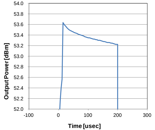
Figure 8. b) f=3.1GHz
