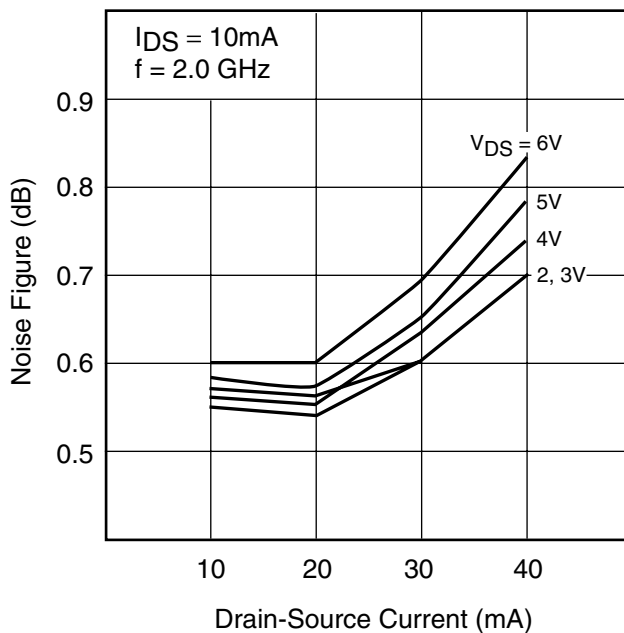
NOISE FIGURE vs. DRAIN-SOURCE CURRENT
