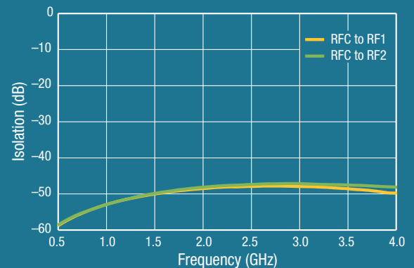
SKY13522-644LF Typical Isolation
